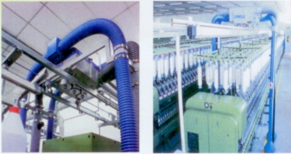
Overhead Travelling Cleaner (Belt Type and Bus Bar Type)
