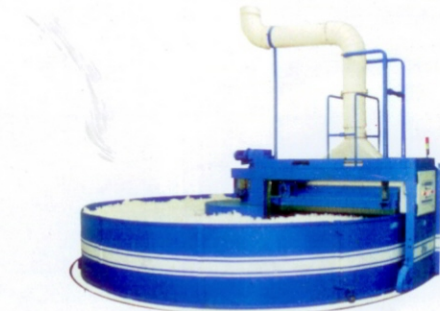
Rotating Automatic Bale Plucker
