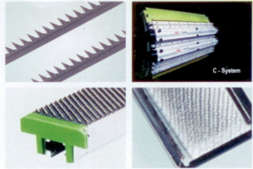
Complete Card Clothing
